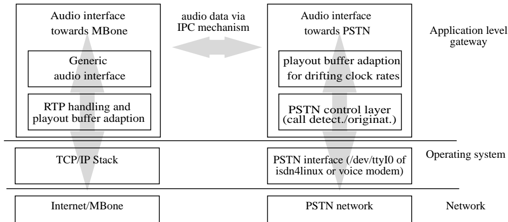
Fig. 3. Audio Forwarding – Components and Data Flow
