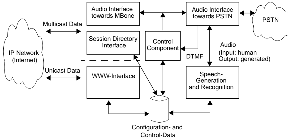
Fig. 2. Architecture of the MBone2Tel Gateway
