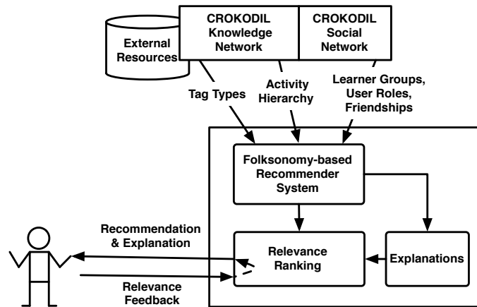
Fig. 1. Conceptual Design of a Personalized Recommender System
