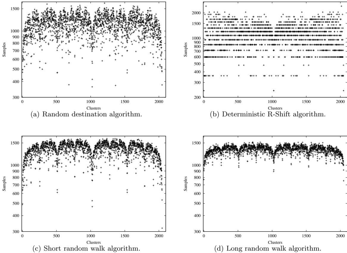
Figure 5. Sampling distribution using random walks.
