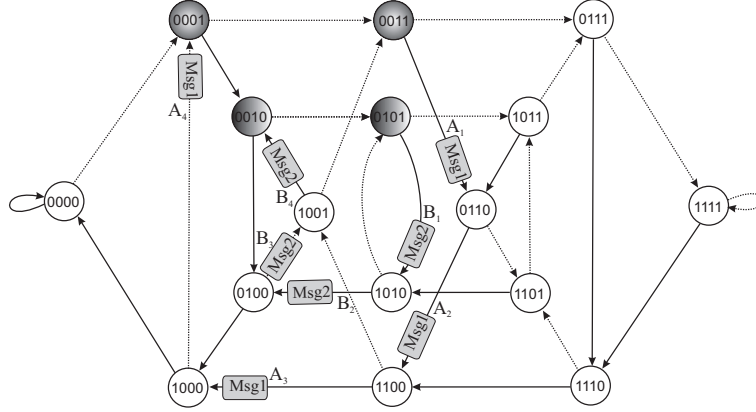
Figure 4. Deterministic R-Shift algorithm.
