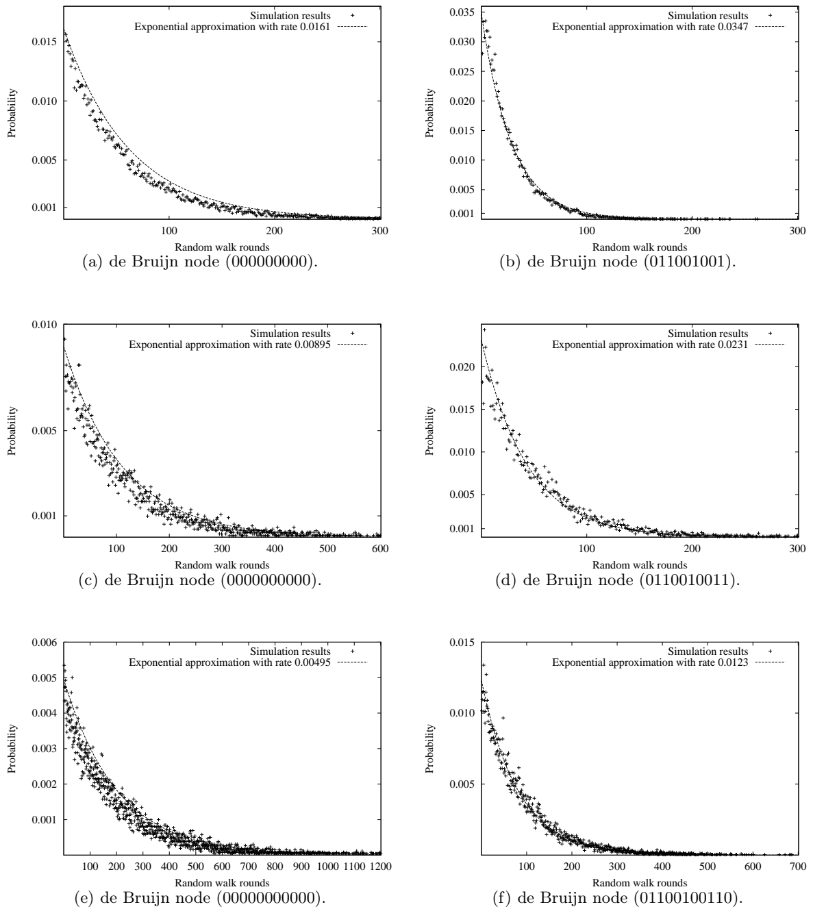
Figure 7. Cluster sampling inter-arrival distribution.
