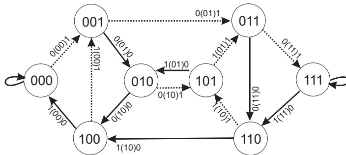
Figure 1. Directed de Bruijn(2, 3) graph.
