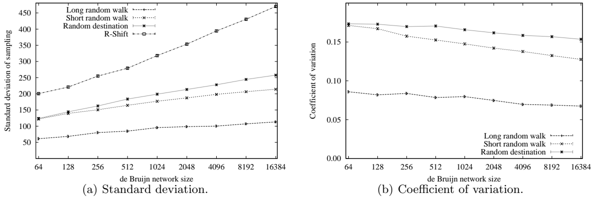
Figure 6. Cluster sampling in de Bruijn networks.
