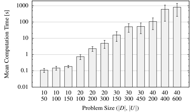
Figure 1: Mean computation times of CDCSP-EXA.KOM, depending on the problem size (with 95% confidence intervals; sample size n = 50 ). Please note the logarithmic scale of the ordinate.
