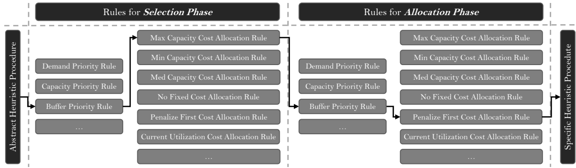
Figure 2: Deduction of Specific Heuristic Approaches
