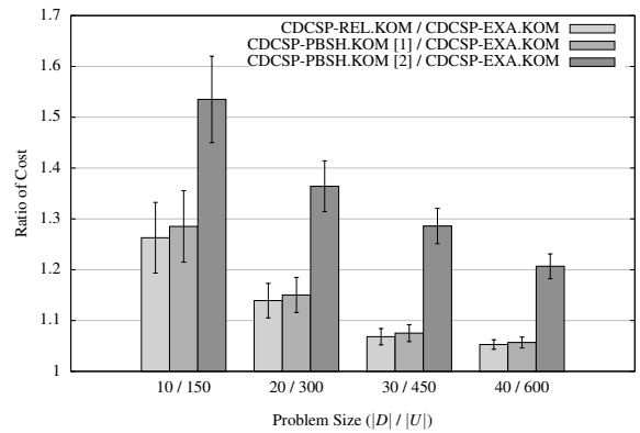
Figure 4: Solution Quality (Small Test Cases)
