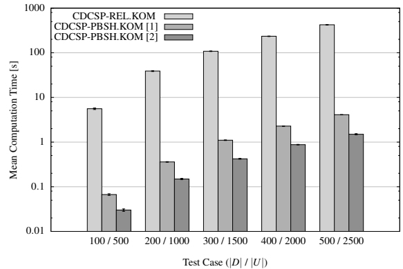
Figure 5: Computation Time (Large Test Cases)
