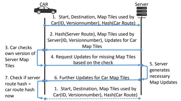
Figure 4: The map exchange protocol sequence.
