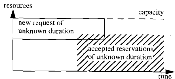
Figure 1: Scheduling of Advance Reservations
