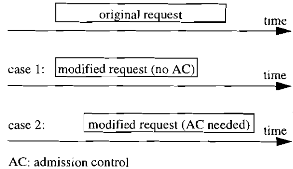
Figure 4: Modification of reservation requests
