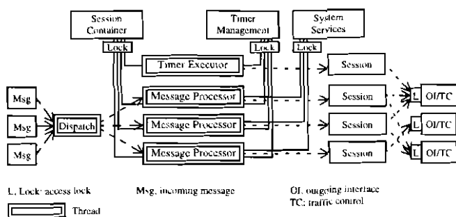
Fig. 3. Multi-threaded message processing.
