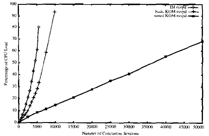
Fig. 5. Performance curve for ISI and KOM rsvp.
