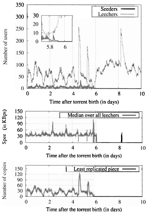
Fig. 2. Snapshot from a torrent in our microscopic trace.
