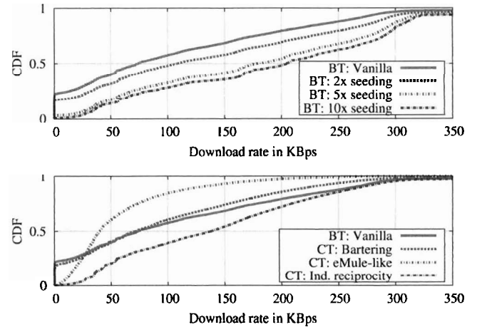
Fig. 7. Cumulative distribution functions (CDF) of the measured download rates. Top: Variants with lengthened seeding times. Bottom: Cross-torrent approaches.
