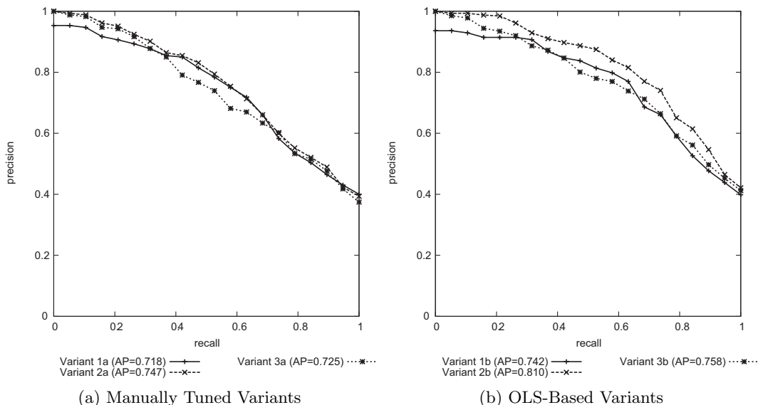
Figure 2: Recall-Precision Curves
