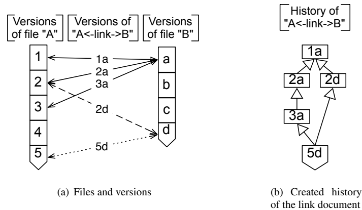
Figure 2: Concurrent updates on a linkdocument
