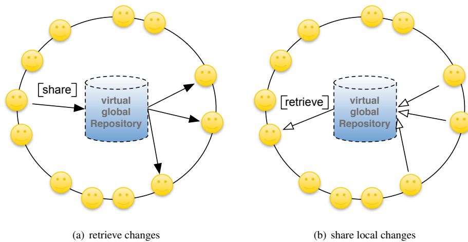
Figure 1: Sharing and retrieving versions using PlatinVC
