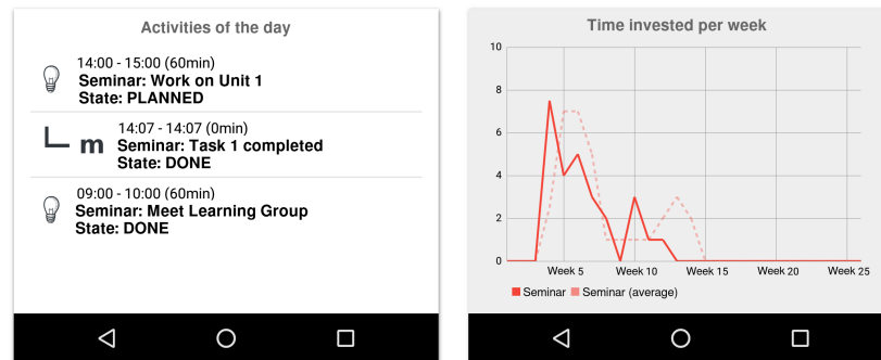
Fig. 2. User-Interface of the learning diary application. The left picture shows the list of learning activities entered into the learning diary application or recognized from Moodle. The right picture shows the visualization of own and peers' weekly invested time in the course.
