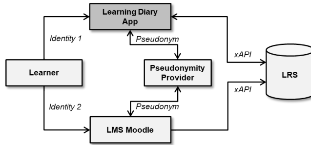
Fig. 1. The proposed architecture, including the learning diary application, Moodle, a central LRS and a component for identity management ( Pseudonymity Provider ).
