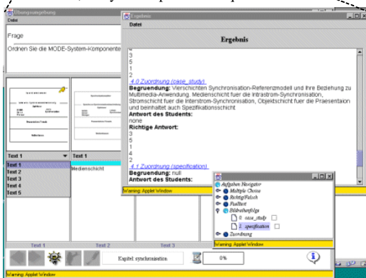
Figure 2: Steps taken by the exercise environment applet to setup an exercise session.
