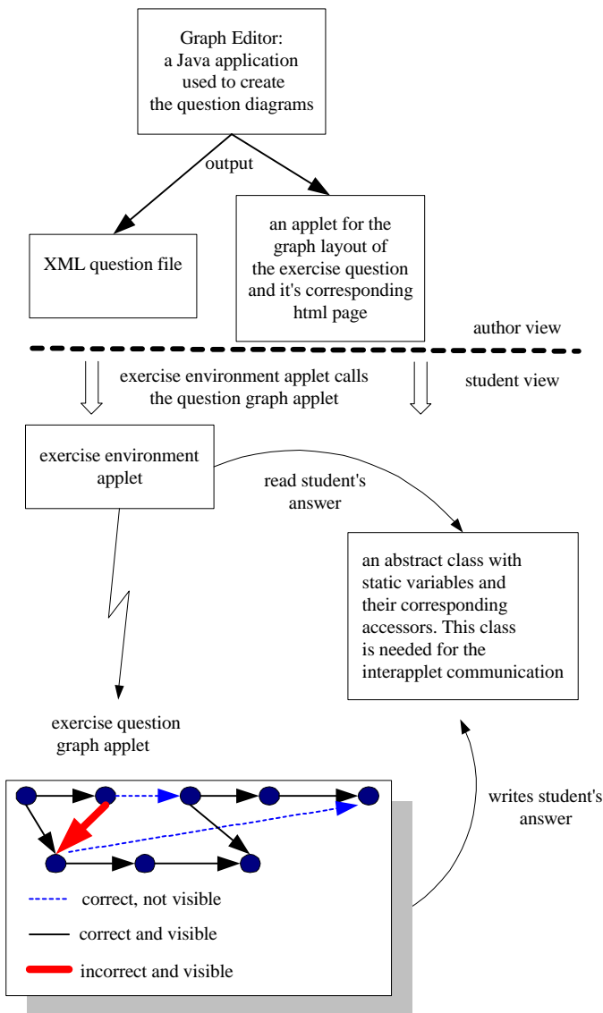
Figure 3: Concept of the question graph applet
