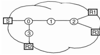
Figure 6: Example of an Unordered Optimal Partition.
