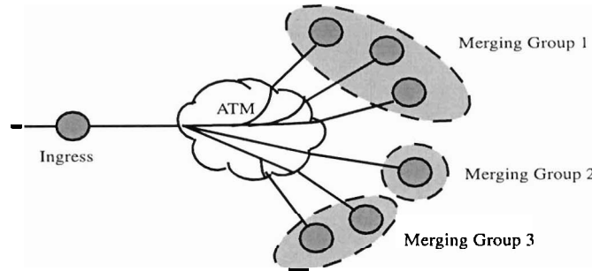
Figure 7: Merging Groups.
