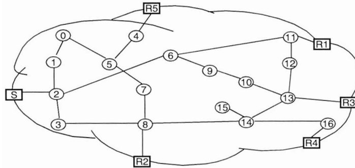
Figure 5: Example Network.
