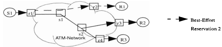
Figure 2: The Limited Heterogeneity Model.
