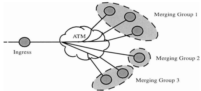
Figure 7: Merging Groups.
