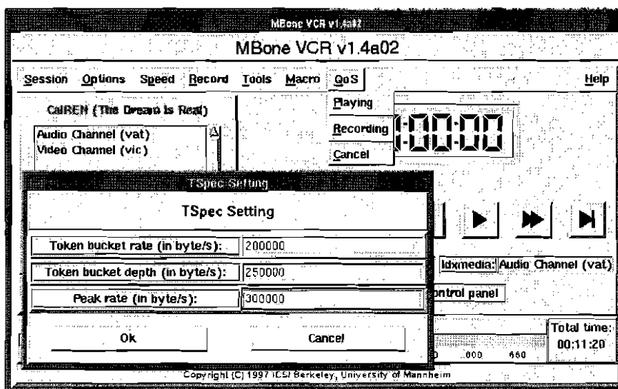
Figure 6: User Interface of the Extended VCR.
