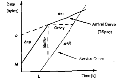
Figure 1: Network calculus for LR schedulers.
