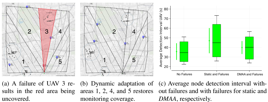
Figure 2: Dynamic Monitoring Area Allocation improves resilience against UAV failures.
