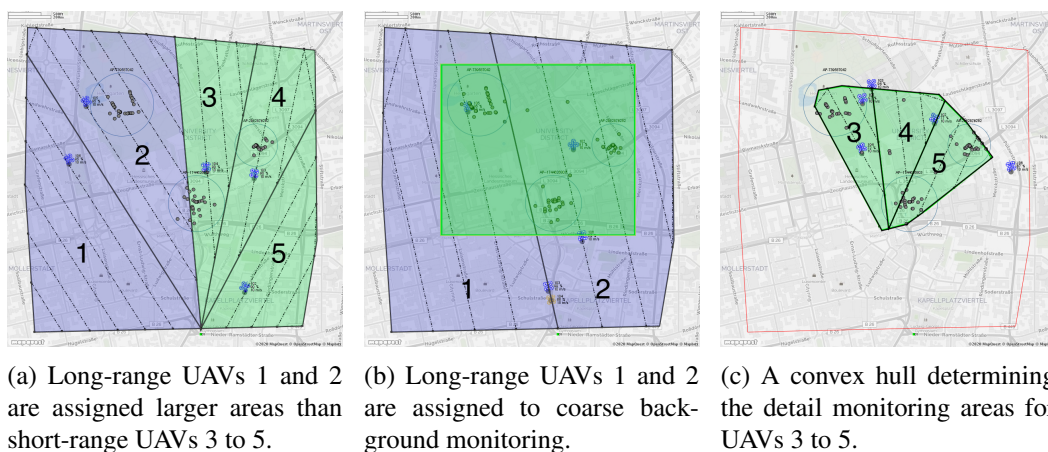
Figure 1: DMAA with adaptation to the encountered node topology. UAVs are represented by blue symbols, smart devices by grey dots, lines represent UAV flight paths.
